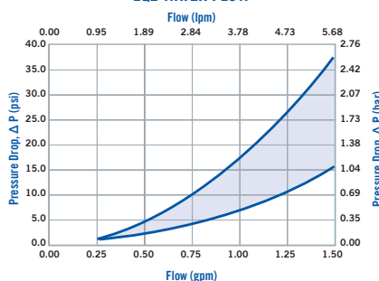
LQ2 WATER FLOW
